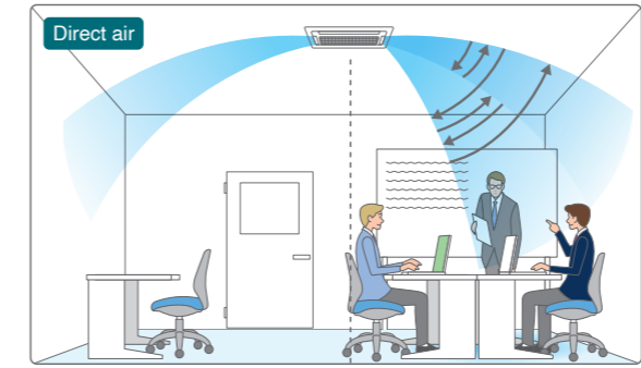
Optimal air direction by "Auto" Swing (narrow)
