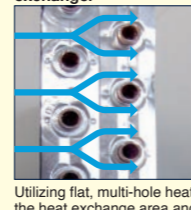
Utilizing flat, multi-hole heat exchanger tubes increases the heat exchange area and realizes energy savings.
