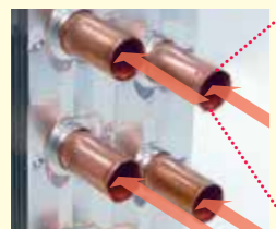
Flow of refrigerant
